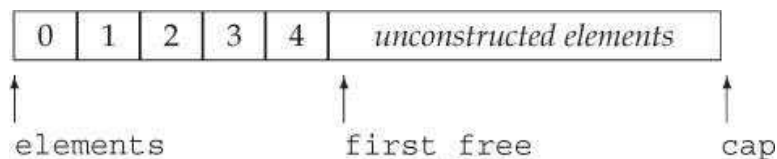
Figure 13.2. StrVec Memory Allocation Strategy
