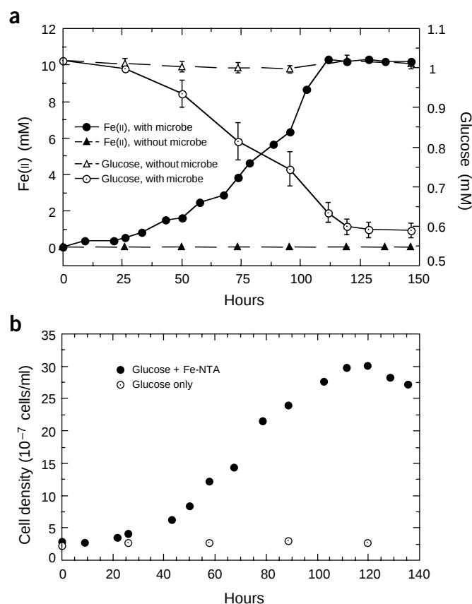
Figure 1 Growth of R. ferrireducens at 25 °C with glucose as electron donor and Fe(III) as the electron acceptor. (a) Glucose consumption and Fe(III) reduction. (b) Cell growth.
