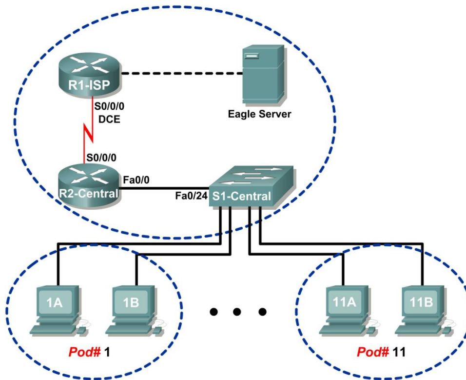
Figure 5. Topology Diagram
