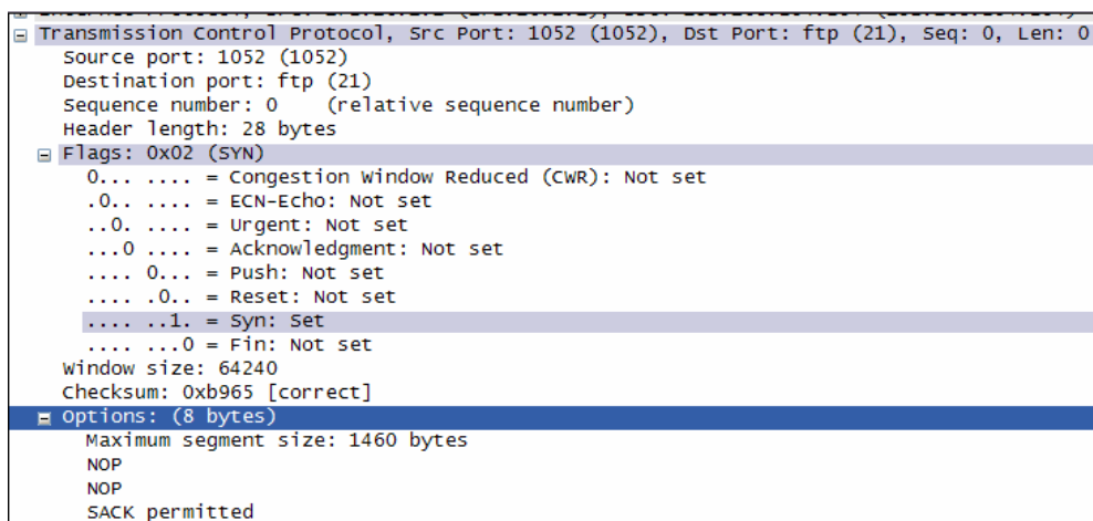
Figure 3. Wireshark capture of a TCP datagram.
